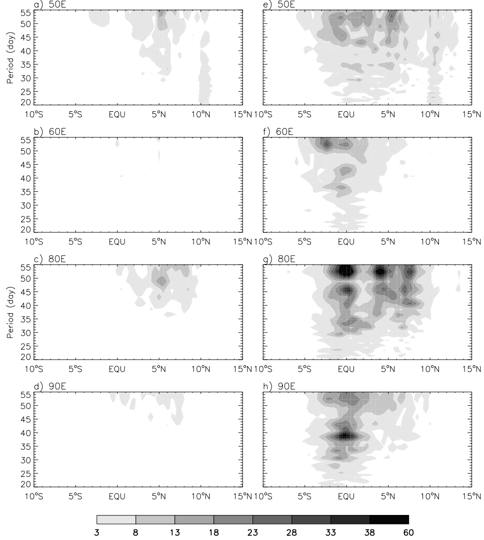
Figure 17: a) Variance spectra of zonal surface currents u_0 along 50^\circ\text{E} from the OGCM_BR, the solution forced by monthly forcing fields; b) Same as a) except for 60^\circ\text{E} ; c) Same as a) except for 80^\circ\text{E} ; d) Same as a) except for 90^\circ\text{E} ; e) Same as a) except for solution OGCM_MR, the solutions forced by the 3-day mean forcing fields; f) Same as e) except for 60^\circ\text{E} ; g) Same as e) except for 80^\circ\text{E} ; h) Same as e) except for 90^\circ\text{E} . Units: \text{cm}^2\text{s}^{-2} .
