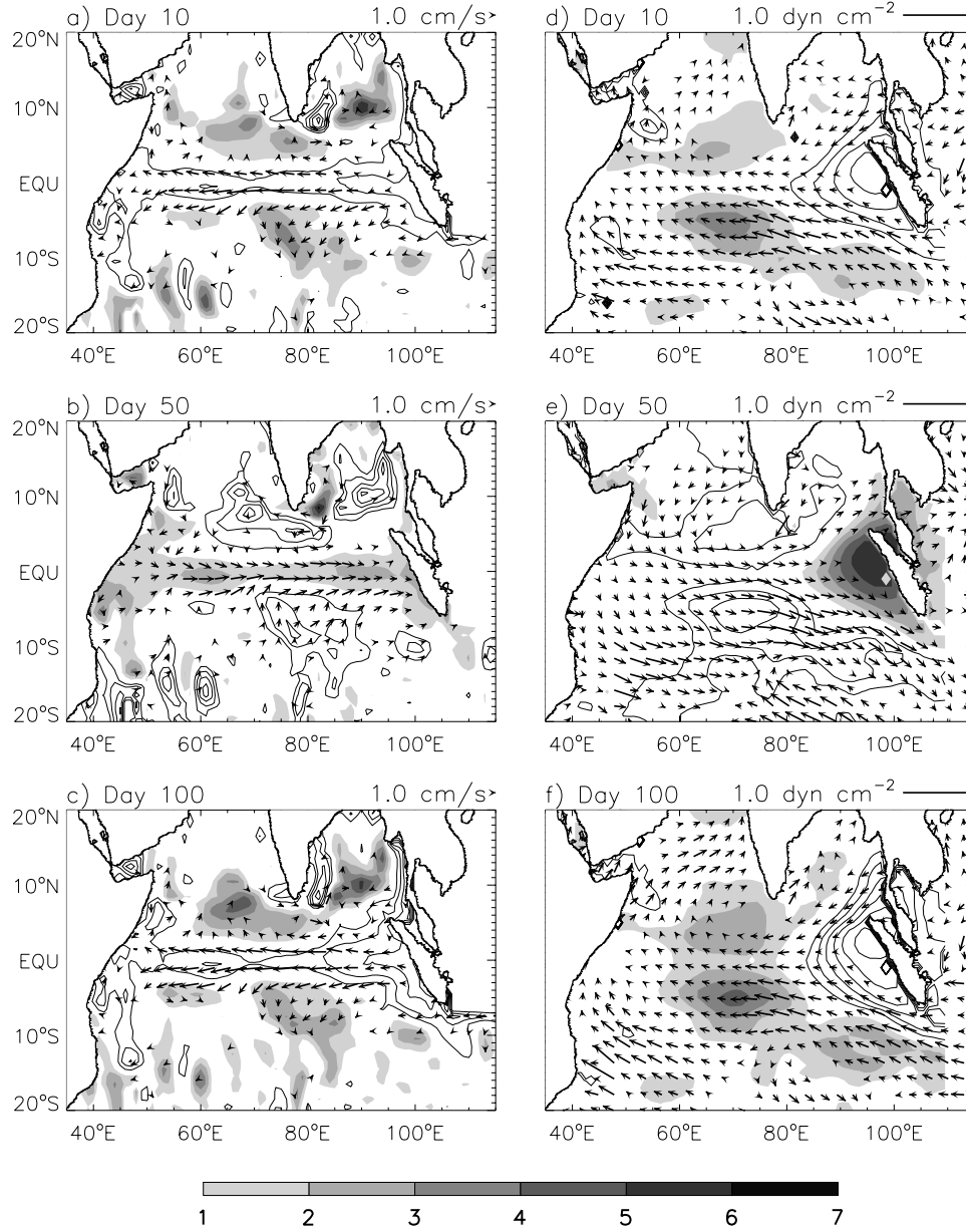
Figure 8: a) The 90-day SLA (fill and line contours) and 90-day surface currents (arrows) for day 10 of 1997; b) Same as a) except for day 50 of 1997; c) Same as a) except for day 100 of 1997; d) The 90-day NCEP windstress (arrows) and 90-day TOPEX/POSEIDON altimeter data (fill and line contours); e) Same as d) except for day 50 of 1997; f) Same as d) except for day 100 of 1997. Units for SLA are cm, for currents are cm s -1 , and for windstress are dyn cm -2 . Positive values for SLA are shaded and negative ones are contoured, with an interval of 1 cm. Zero contours are suppressed.
