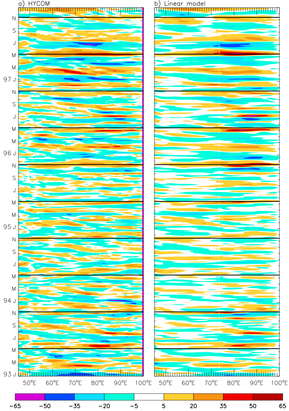
Figure 5: a) Longitude-time plot of intraseasonal component for zonal current in the surface mixed layer, u_m , along the Indian Ocean equator (averaged over 2°S–2°N) from solution OGCM_MR for the period of 1993–1997, the solution that includes all intraseasonal forcing; b) Same as a) except for intraseasonal zonal currents averaged in the upper 20 meters from LM_MR. Units: \text{cm s}^{-1} .
