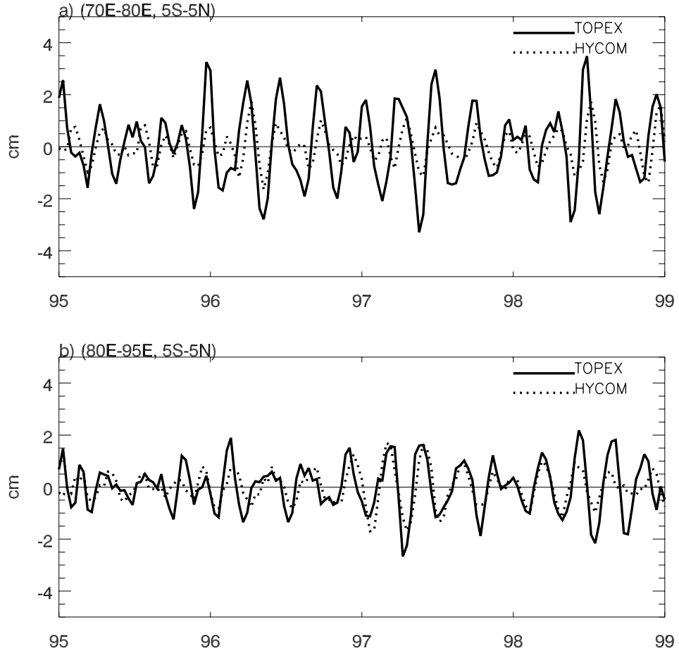
Figure 4: a) Time series of intraseasonal SLA during 1995-1998 averaged over the central equatorial basin ( 70^{\circ}\text{E} - 80^{\circ}\text{E} , 5^{\circ}\text{S} - 5^{\circ}\text{N} ) from TOPEX/POSEIDON altimeter data (solid curve) and from the OGCM_MR (dotted curve); b) Same as a) except for averaging over the eastern basin ( 80^{\circ}\text{E} - 95^{\circ}\text{E} , 5^{\circ}\text{S} - 5^{\circ}\text{N} ). Units: cm.
