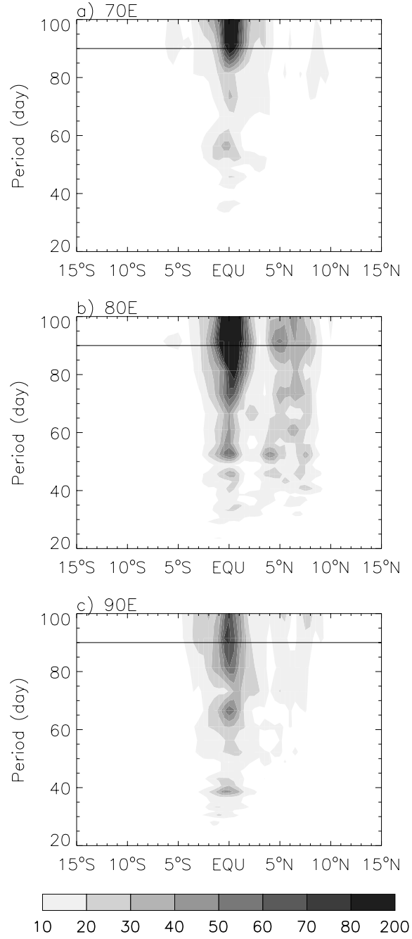
Figure 7: a) Meridional section at 70°E for the variance spectra of 3-day mean zonal surface currents from solution OGCM_MR, based on the solutions for the period of 1990-2001; b) Same as a) except for meridional section at 80°E; c) Same as a) except for meridional section at 90°E. Units: \text{cm}^2\text{s}^{-2} .
