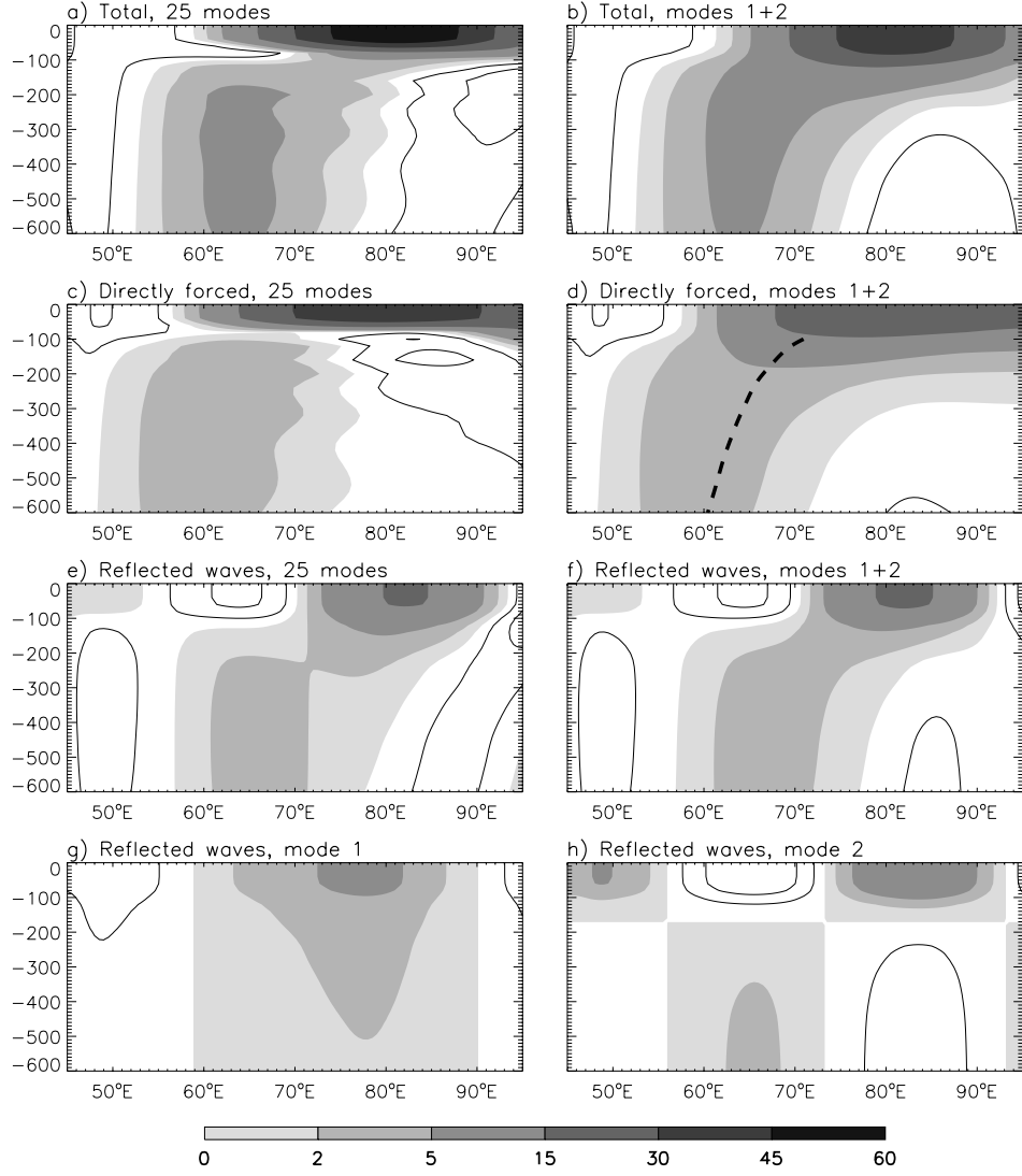
Figure 14: Vertical sections of zonal current u above 600 m along the Indian Ocean equator ( 1^\circ\text{S} - 1^\circ\text{N} average) from the idealized solution at the 90-day period (Figure 11). a) Total solution, 25 modes; b) Total solution, first 2 modes; c) Directly forced response, 25 modes; d) Directly forced response, first 2 modes; the dashed curve shows the WKB ray path for l = 1 Rossby waves at the 90-day period; e) Reflected waves, 25 modes; f) Reflected waves, first 2 modes; g) Reflected waves, mode 1; h) Reflected waves, mode 2. Units: \text{cm s}^{-1} .
