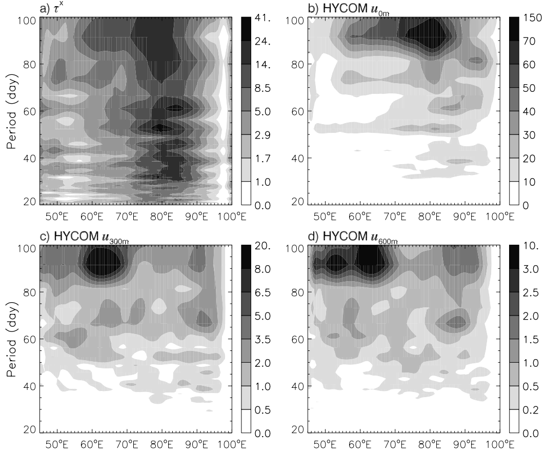
Figure 6: a) Variance spectra for 3-day mean NCEP/NCAR zonal windstress along the Indian Ocean equator (averaged over 2°S-2°N), based on a 12-year record (1990-2001). Variance at periods of 20–100 days is plotted. Units: 10^{-6}\text{dyn}^2\text{cm}^{-4} ; b) Same as a) except for variance spectra for 3-day mean zonal surface mixed-layer currents from OGCM_MR. Units: \text{cm}^2\text{s}^{-2} ; c) Same as b) except for 300 m depth; d) Same as b) except for 600 m depth.
