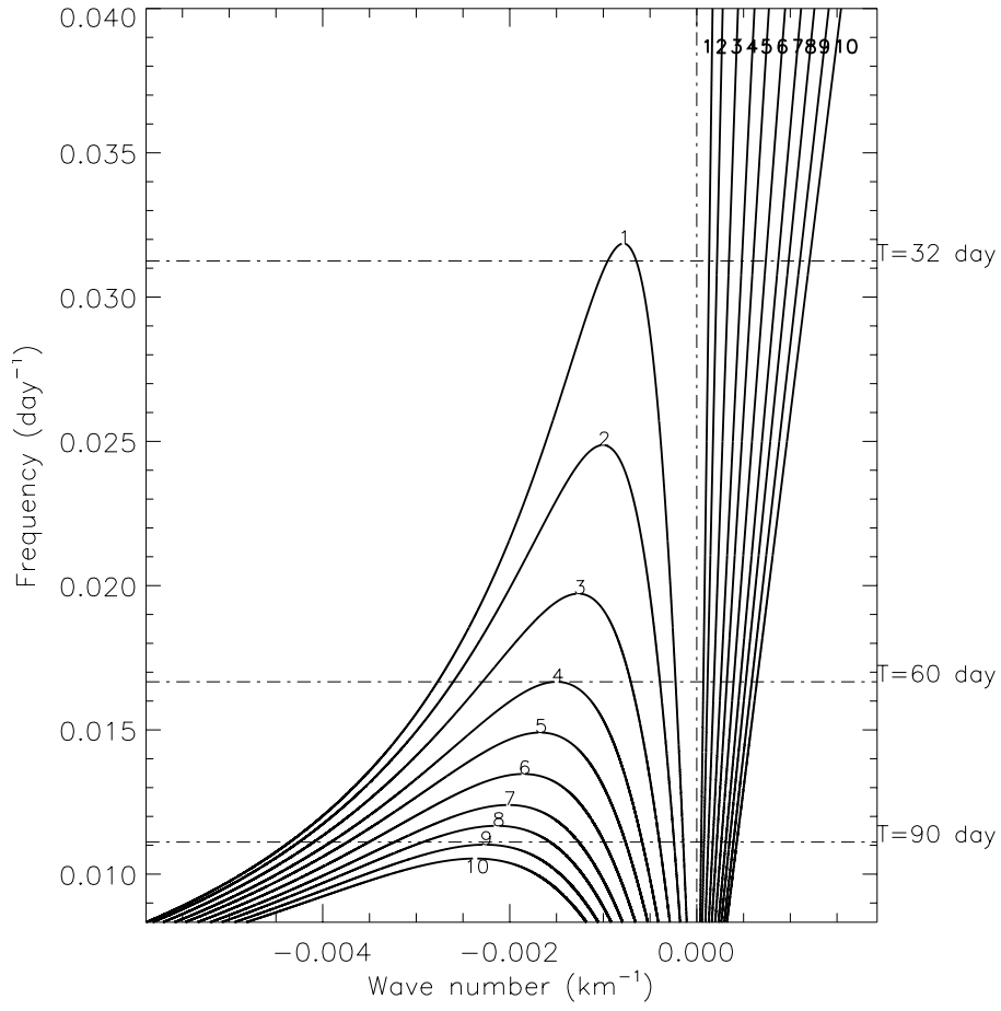
Figure 12: Dispersion curves of Kelvin and l = 1 Rossby waves for the first 10 baroclinic modes ( n=1, 2, \dots, 10 ).
