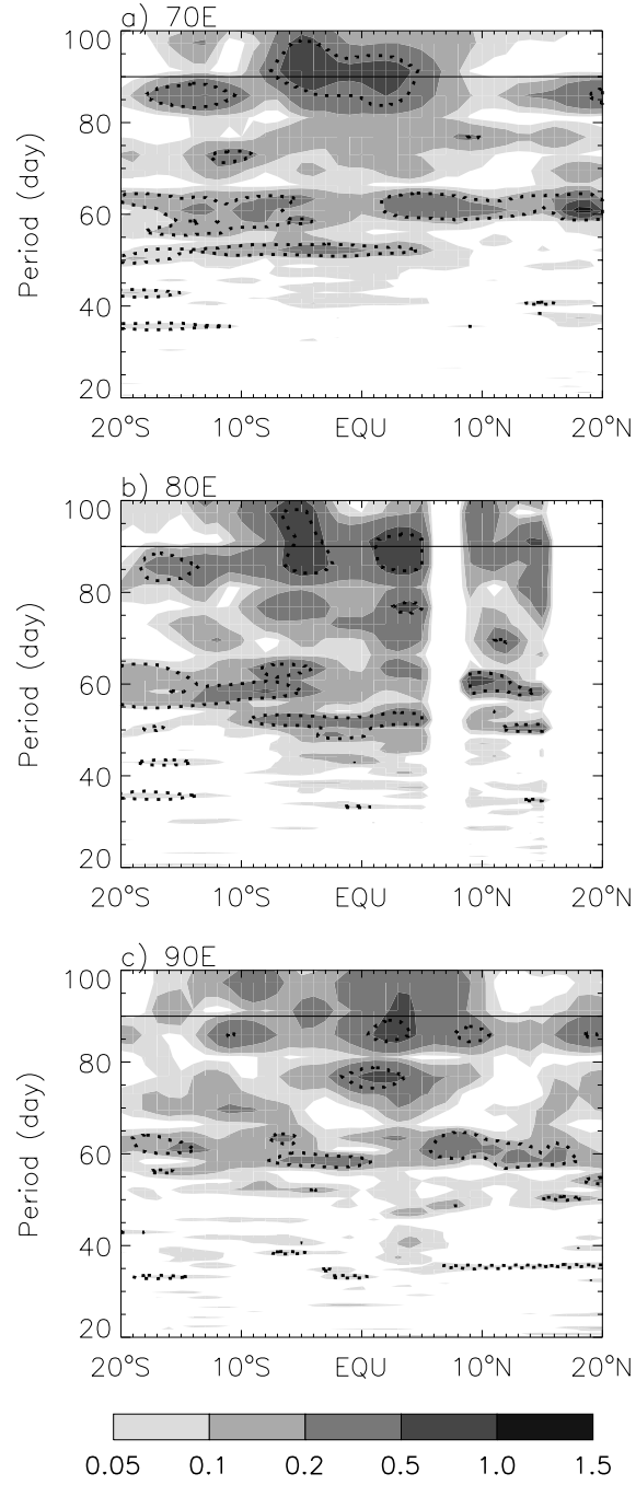
Figure 1: a) Meridional section for variance spectra of TOPEX/POSEIDON sea level anomaly (SLA) along 70°E, based on a 8-year record (1993–2000) with a 10-day resolution; b) Same as a) except for the section along 80°E; c) Same as a) except for the section along 90°E. Units: \text{cm}^2 . Dashed contours are the 95% significance level. The 90-day and most 30-60 day spectral peaks are above 95% significance.
