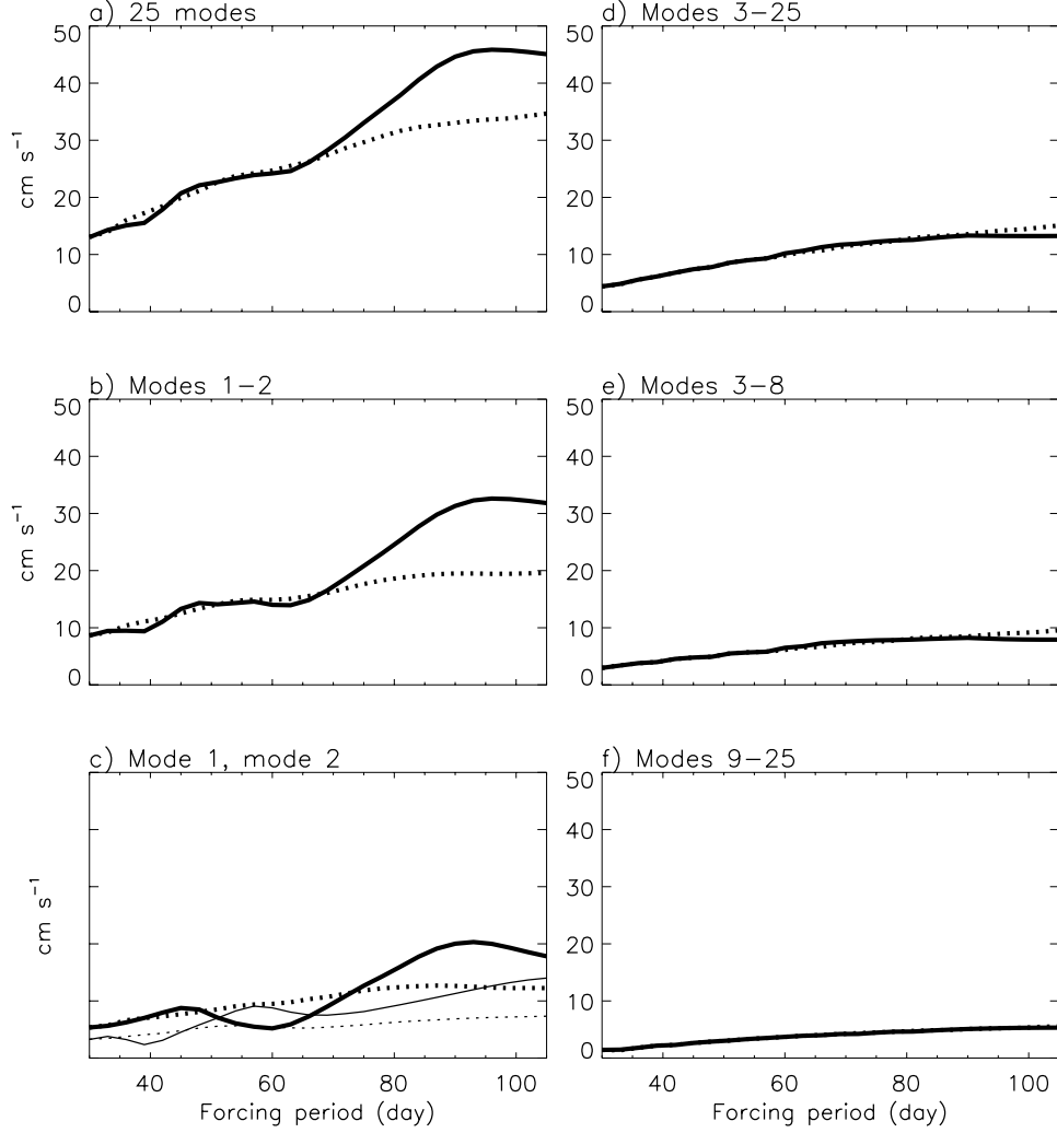
Figure 11: Amplitudes of zonal surface currents from a series of experiments forced by a series of idealized zonal windstress (See text for detail). The winds have the same amplitudes and spatial structure for each experiment and differ only in frequency, which varies from period of 30 days to 105 days for every 3-day interval. a) Sum of the first 25 baroclinic modes for the total solution (solid curve) and for the directly forced response (dotted curve); b) same as a) except for sum of the first 2 baroclinic modes; c) same as a) except for mode 2 (thick curves) and mode 1 (thin curves); d) same as a) except for sum of modes 3-25; e) same as a) except for sum of modes 3-8; f) same as a) except for sum of modes 9-25. Units: \text{cm s}^{-1} .
