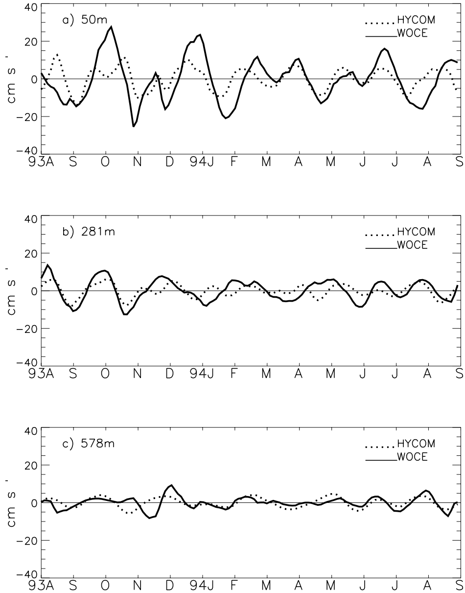
Figure 3: a) Intraseasonal components of zonal currents in the central equatorial Indian Ocean ( 80.5^{\circ}\text{E}, 0^{\circ}\text{N} ) observed by WOCE current meter data during August 1993-August 1994 at 50 m depth (solid curve), and intraseasonal currents from OGCM_MR at the same depth (dotted curve); b) Same as a) except for currents at 281 m depth; c) Same as a) except for currents at 578 m depth. Units: \text{cm s}^{-1} .
