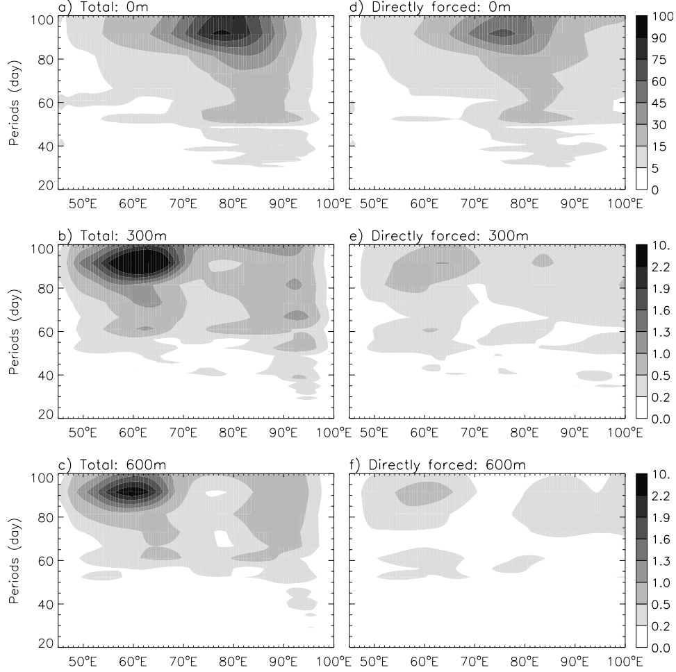
Figure 10: a) Variance spectra along the Indian Ocean equator (averaged over 1^\circ\text{S} - 1^\circ\text{N} ) for 3-day mean zonal currents from LM_MR at the surface, based on the solutions for the period of 1990-2001; b) Same as a) except for 300 m depth; c) Same as a) except for 600 m; d) Same as a) except for solution LM_FR, which estimates directly forced response that is independent of Rossby waves reflected from the eastern ocean boundary; e) Same as d) except for 300 m depth; f) Same as d) except for 600 m. Units: \text{cm}^2\text{s}^{-2} .
