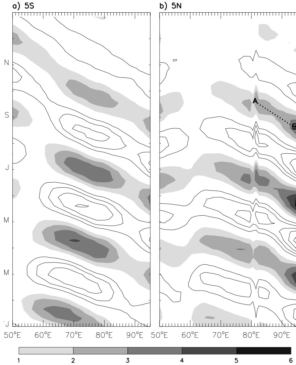
Figure 9: a) Longitude-time plot of 90-day SLA from TOPEX/POSEIDON satellite altimetry data during 1997 at 5°S; b) Same as a) except for at 5°N. Units: cm.
