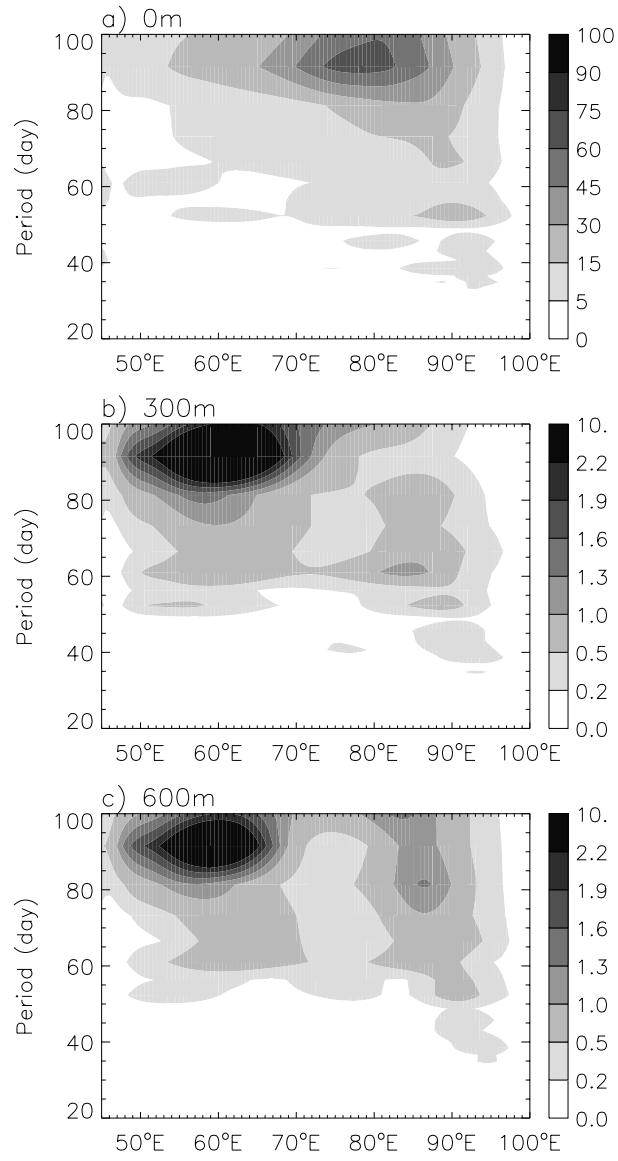
Figure 13: Same as Figure 10 (left panels) except for the first two baroclinic modes response. Units: \text{cm}^2\text{s}^{-2} .
