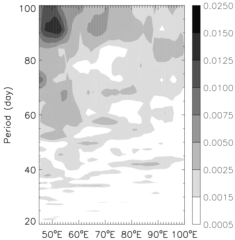
Figure 16: Variance spectra of Reynolds weekly SST along the Indian Ocean equator based on the period of 1982-2002. Units: °C 2 .
