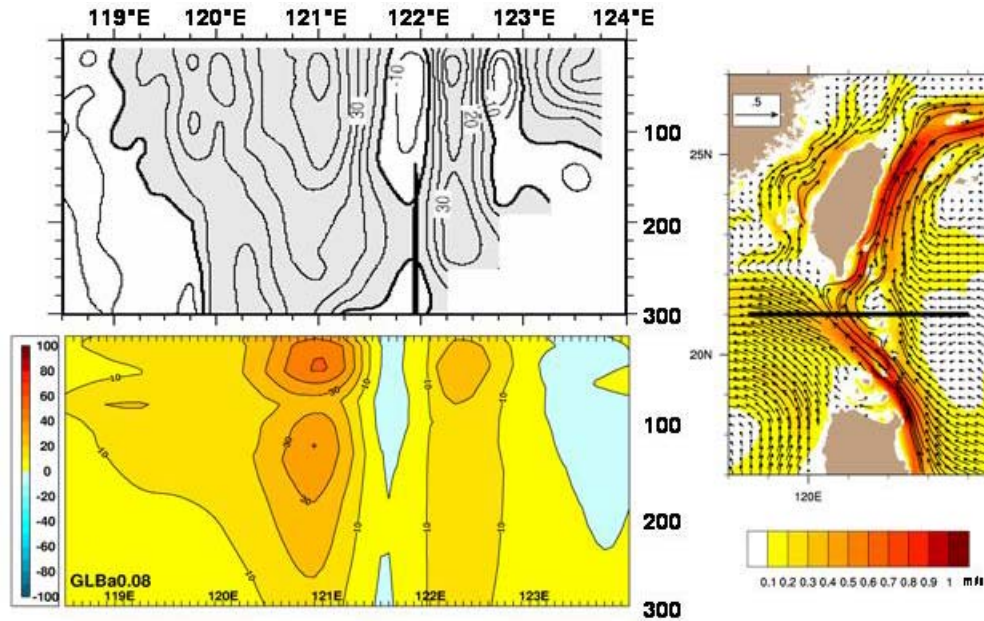
Figure 3: (Right) Mean upper layer currents in Luzon Strait from 1/12^\circ global HYCOM using climatological wind and thermal forcing from the ECMWF. (Left – top) Mean meridional velocity in the upper 300 m based on a ten-year composite of shipboard acoustic Doppler current profiler data from Liang et al. (2003) and (left – bottom) from global HYCOM. Both observed and simulated currents indicate a split Kuroshio with a stronger western than eastern branch and weak counterflow in the lee of the Babuyan Island chain. The black line indicates the location of the vertical cross-section.
