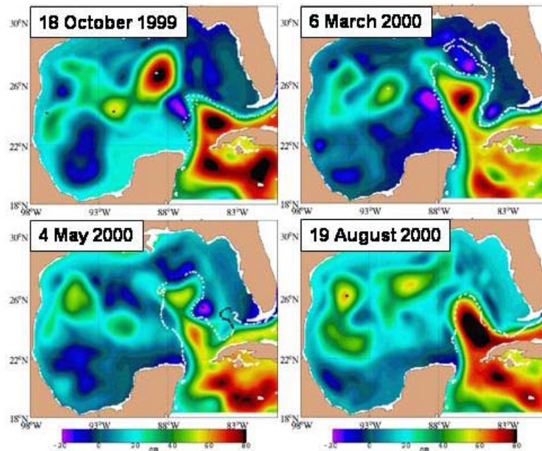
Figure 5: Nowcast SSH at four dates from 1/12^\circ Gulf of Mexico HYCOM using the NCODA scheme. The HYCOM-NCODA cycling system assimilates SSH at altimeter ground tracks, MCSST and XBT profile data. Overlaid are frontal locations based on MCSST data and produced by NAVOCEANO. Isolated points define eddy centers. White (black) lines or points are newer (older) than four days.
