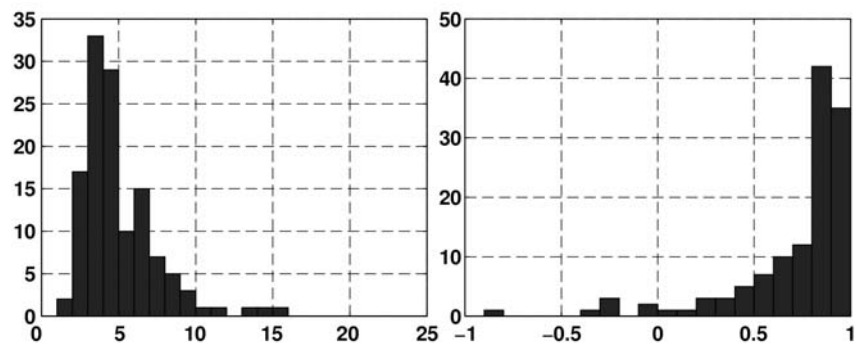
Figure 4: Histograms of (left) root mean square difference and (right) correlation coefficient between 126 observed coastal and island sea level stations and 1/12° global HYCOM using 3-hourly FNMOC NOGAPS wind and thermal forcing for 2003. A 30-day running average is applied to all time series. The median rms difference is 4.4 cm and the median correlation coefficient is .85.
