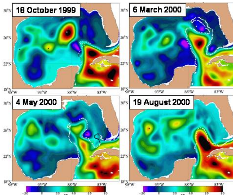
Figure 5: Nowcast SSH at four dates from 1/12^\circ Gulf of Mexico HYCOM using the NCODA scheme. The HYCOM-NCODA cycling system assimilates SSH at altimeter ground tracks, MCSST and XBT
