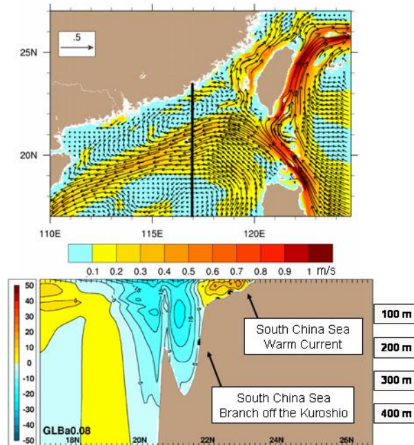
Figure 1: (Top) Mean upper layer currents in the northern South China Sea (SCS) from 1/12^\circ global HYCOM using climatological wind and thermal forcing from the ECMWF. Note the across shelf flow as the SCS branch off the Kuroshio feeds the northeastward-directed SCS Warm Current along the Chinese coast, which flows counter to the prevailing northeast to southwest directed monsoon winds. (Bottom) Zonal mean velocity along 117^\circ\text{E} in the upper 500 m with blue = westward and yellow/orange = eastward. HYCOM makes a smooth transition from the deep to shallow water. It is also capable of handling the sharp topographic rise near 21^\circ\text{N} . The black line indicates the location of the vertical cross-section.
